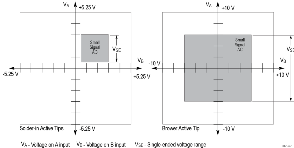
Figure 1: Input dynamic range
