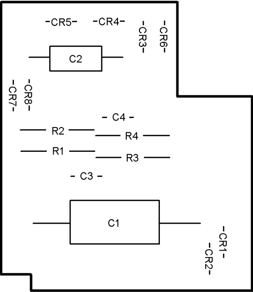
Figure 2-4 A1 Main Board Assembly Component Location
